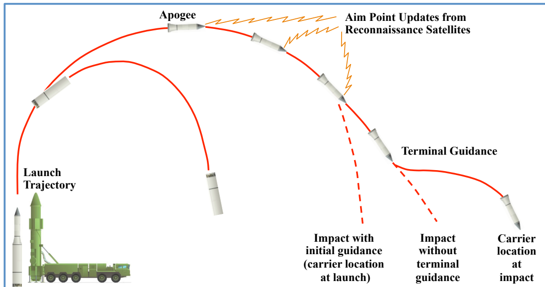
FIGURE 6: PLA ASBM CONCEPT 81
