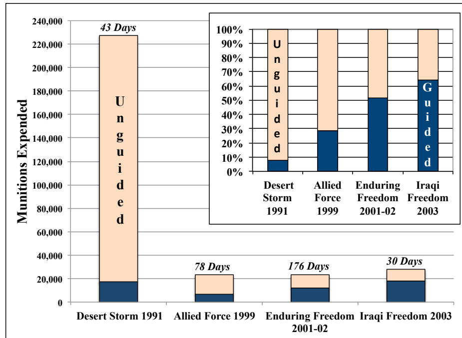
FIGURE 3: U.S. UNGUIDED VERSUS GUIDED MUNITIONS EXPENDITURES IN FOUR AIR CAMPAIGNS 41
