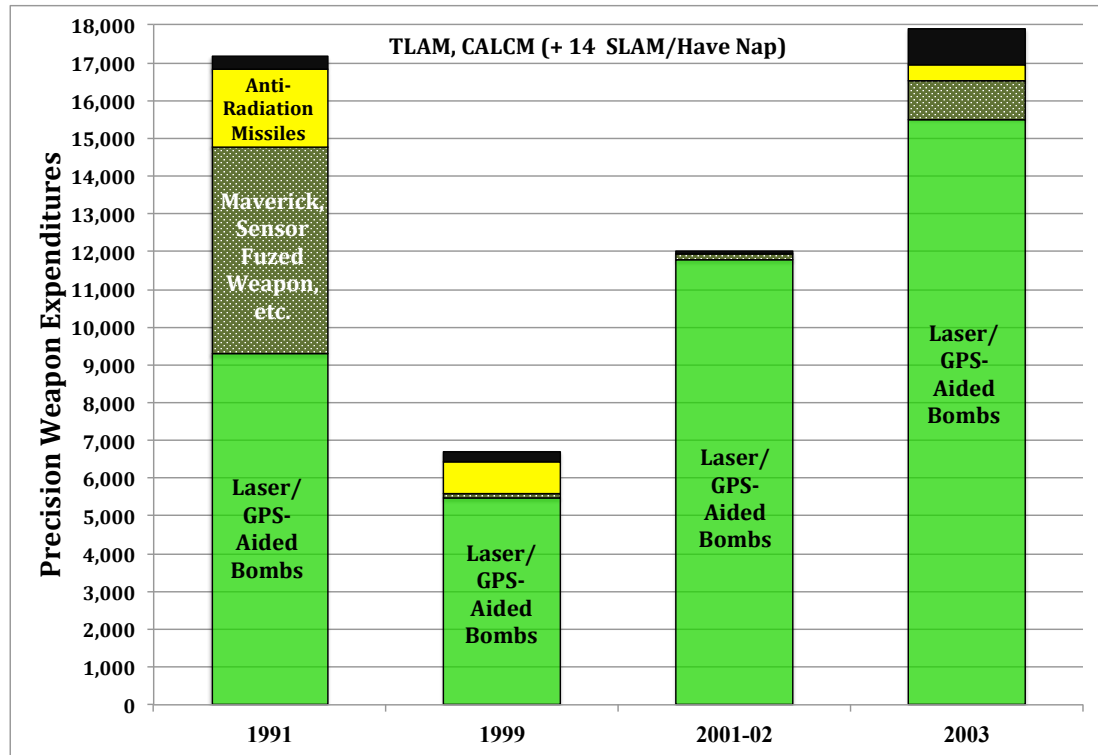
FIGURE 5: U.S. PGM USAGE IN FOUR AIR CAMPAIGNS
